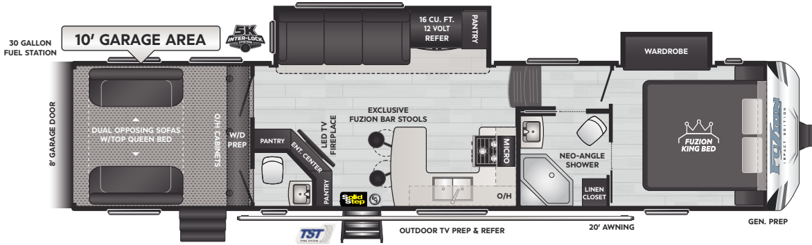
359 | WEIGHT 12915 | LENGTH 39' 0"
