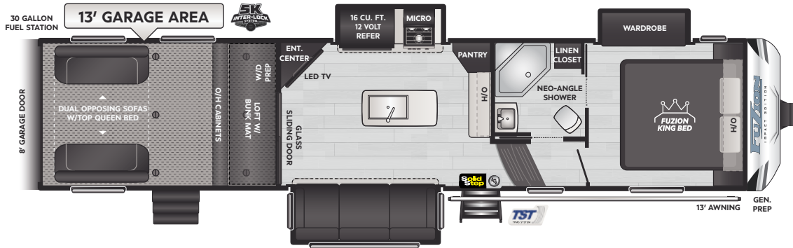
343 | WEIGHT 12694 | LENGTH 39' 0"
